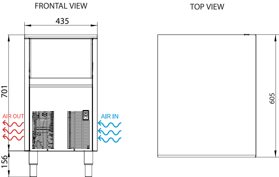
REAR VIEW
